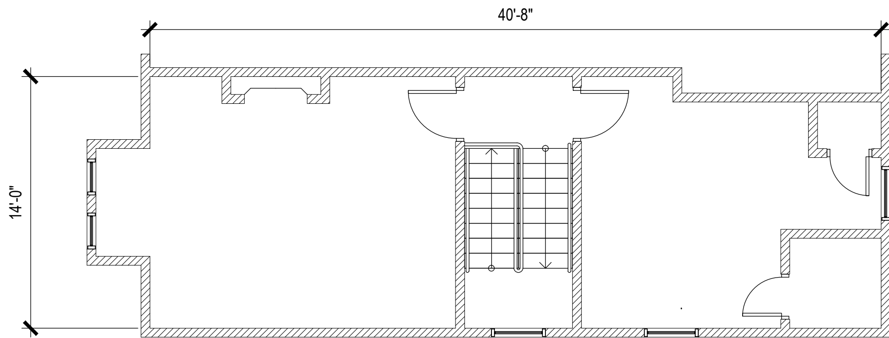
3RD FLOOR
